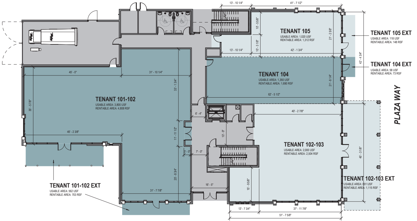
① FIRST FLOOR LEASING PLAN 3/32" = 1'-0"
