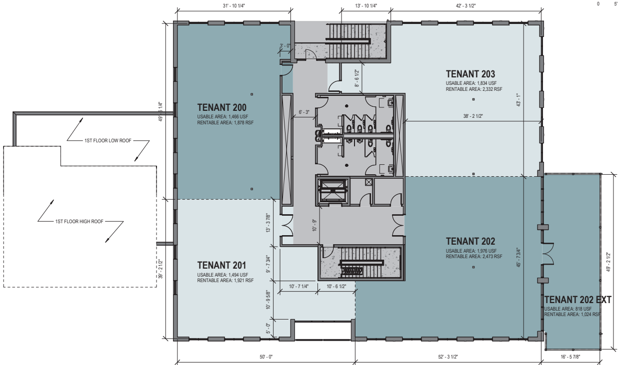
② SECOND FLOOR LEASING PLAN 3/32" = 1'-0"
