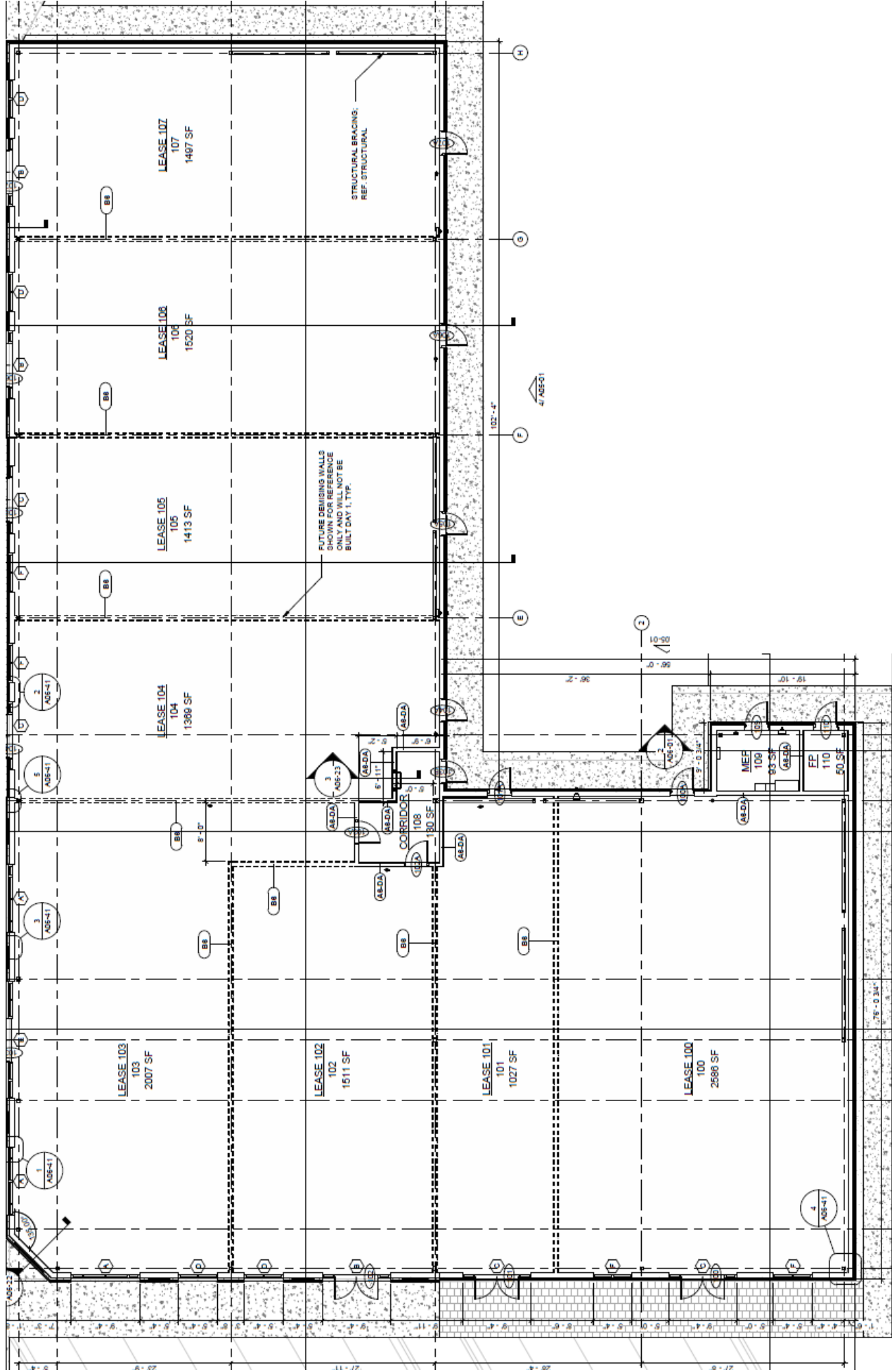
BUILDING 11 | FLOOR PLAN
